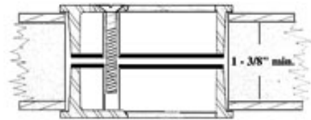
Back-to-Back Pulls for Hollow Core Doors 72075 - BB2 / 72075 - TBI
