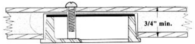
Single Pulls for Hollow Metal 72075 - TBI
